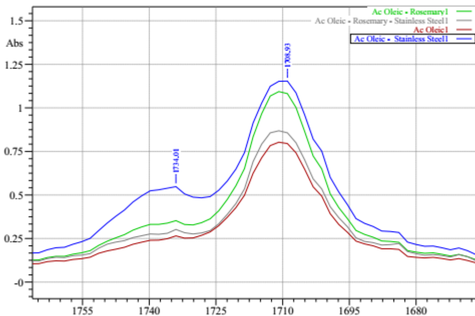
Fig. 2. FTIR Spectra of measured samples
